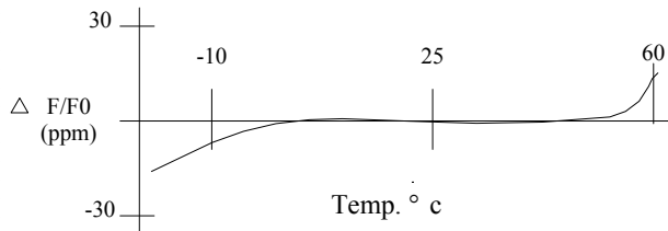
温度曲线图 Temperature Curve
